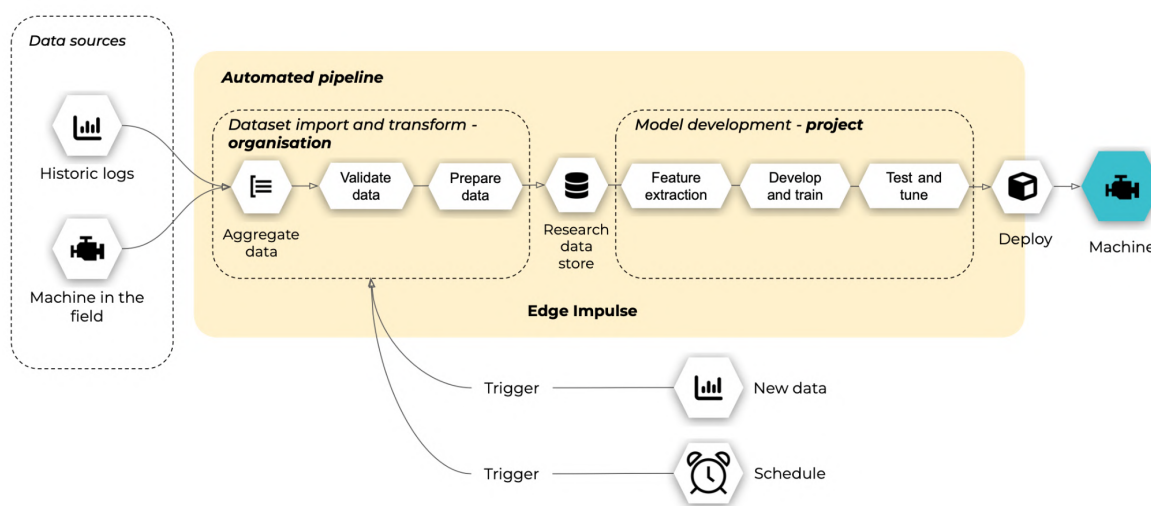
Figure 26: An example end-to-end automated ML flow set up in Edge Impulse
